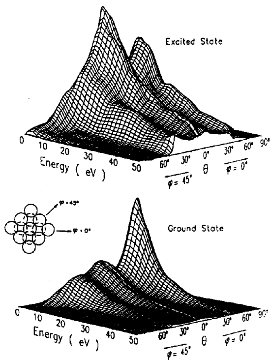
FIG. 1. Energy- and angle-resolved distributions of Rh atoms in the {}^4F_{7/2} excited state and {}^4F_{9/2} ground state, ejected from 5 keV Ar ^+ ion bombarded Rh{100}. The data correspond to ejection along \varphi = 0^\circ ( \langle 100 \rangle ) and \varphi = 45^\circ ( \langle 110 \rangle ) crystallographic directions, as defined in the inset. Due to the symmetry of the surface and the angular resolution (e.g., \Delta\varphi = \pm 18^\circ at \theta = 45^\circ ), the results represent the data over \sim 50\% of all space. Both plots are normalized to the maximum intensity peaks. The dashed circles in the inset represent second layer atoms.
