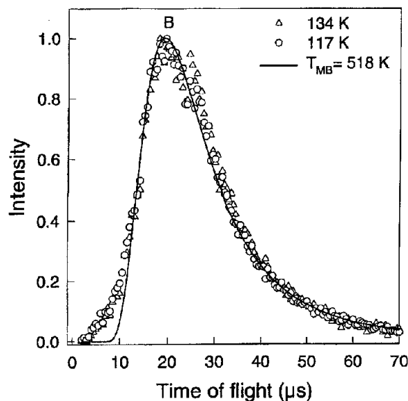
Figure 2. The time-of-flight distribution of neutral benzene molecules for 800 L exposure, at different surface temperatures. The solid line shows a Maxwell-Boltzmann distribution with a fit temperature of 518 K.
