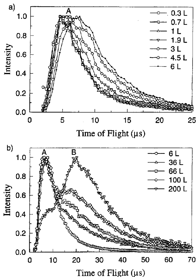
Figure 1. The time-of-flight distributions of neutral benzene molecules for (a) low exposures, (b) high exposures expressed in langmuirs (L). The high and low kinetic energy components are labeled A and B.
