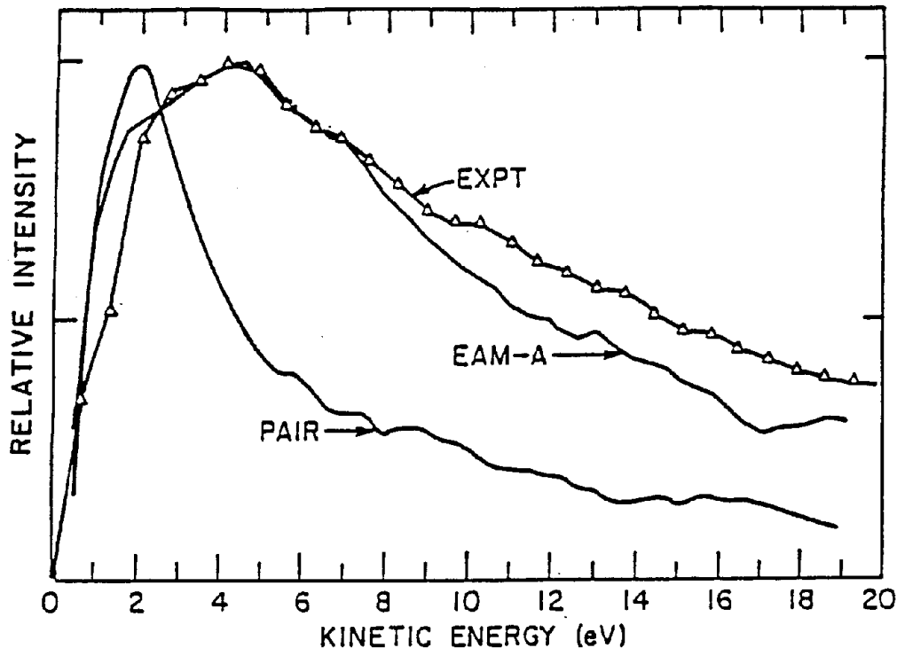
Angle integrated experimental and calculated kinetic energy distributions. In all cases the curves are peak normalized.
