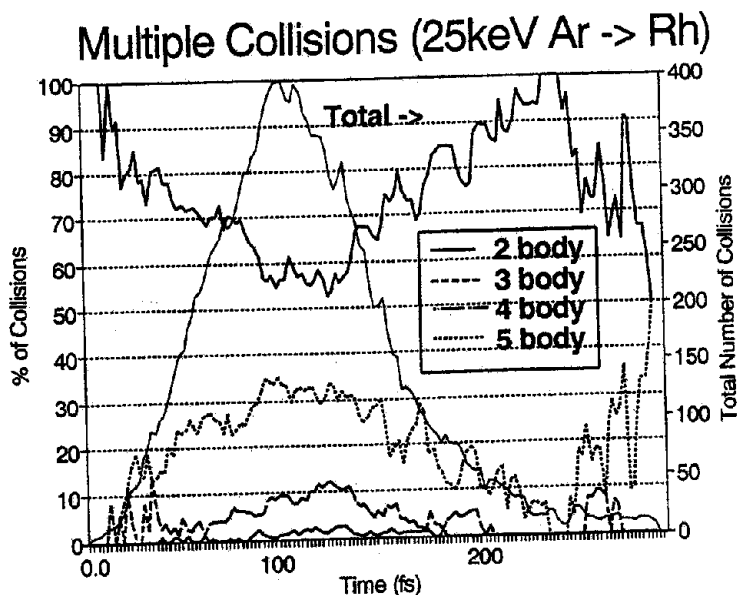
Figure 2. Distribution of multiple collisions as a function of the lifetime of the high activity cascade. A significant number of multiple (more than binary) collisions is observed during the peak activity of the cascade
