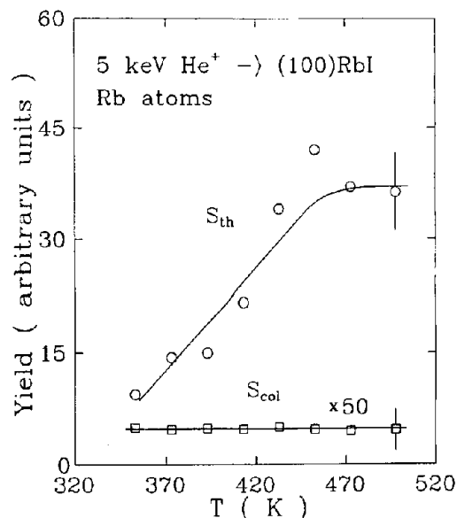
Fig. 2. The temperature dependence of the thermal channel (circles) and the collisional channel (squares) of desorption for 5 keV He + irradiation of RbI (100). The line is drawn only as a visual aid.
