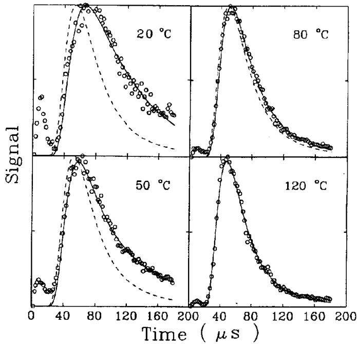
Fig. 1. The TOF spectra measured for 5 keV He + bombardment of RbI {001} at four temperatures. The open circles are the experimental points while the dashed line describes the Maxwell-Boltzmann distribution at the given temperature. The solid line is the obtained fit using Eq. (3).
