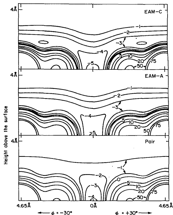
FIG. 4. Contour plots of the potential energy [in eV from Eq. (1)] of a Rh atom ejecting from a Rh{111} surface for the pair potential, EAM-A and EAM-C. The ordinate is the height of the atom above the surface (Å). The abscissa is the position of the atom (Å) along the surface in the \phi = \pm 30^\circ azimuths.
