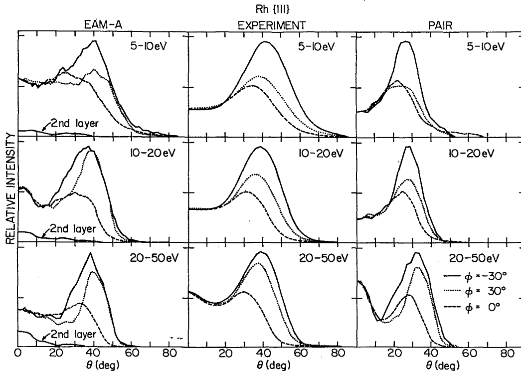
FIG. 3. Polar angle distributions for various azimuthal angles for fixed secondary kinetic energy of the Rh atoms. In each frame the data are normalized to the \phi = -30^\circ peak intensity. For the calculated data the full width at half maximum (FWHM) of the resolution is 15^\circ in the polar angle. A constant solid angle is used in the histogramming procedure. The experimental resolution is approximately the same. The surface normal corresponds to \theta = 0^\circ . The curve marked 2nd layer is the polar distribution along \phi = -30^\circ for the ejected second-layer atoms.
