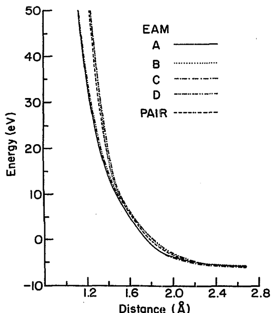
FIG. 5. Energy of an atom in the second layer as a function of the distance to another atom in the second layer for the various potentials. The equilibrium separation is 2.69 Å.
