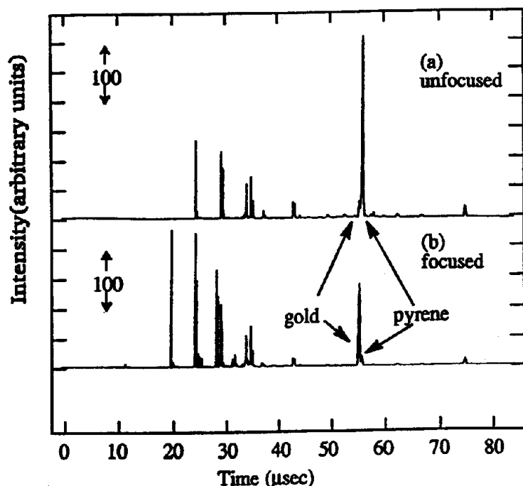
Figure 8. Time-of-flight MPRI spectrum of pyrene indicating the molecular ion at 202 amu for an (a) unfocused and a (b) tightly focused laser beam. The TOF-SIMS spectrum using a 510 ns Ar + ion pulse is shown in (c). The time scale is somewhat arbitrary. The ion pulse occurs at \sim 3 \mu\text{s} , and the laser is activated after 9 \mu\text{sec} . Masses are then computed from known elements.
