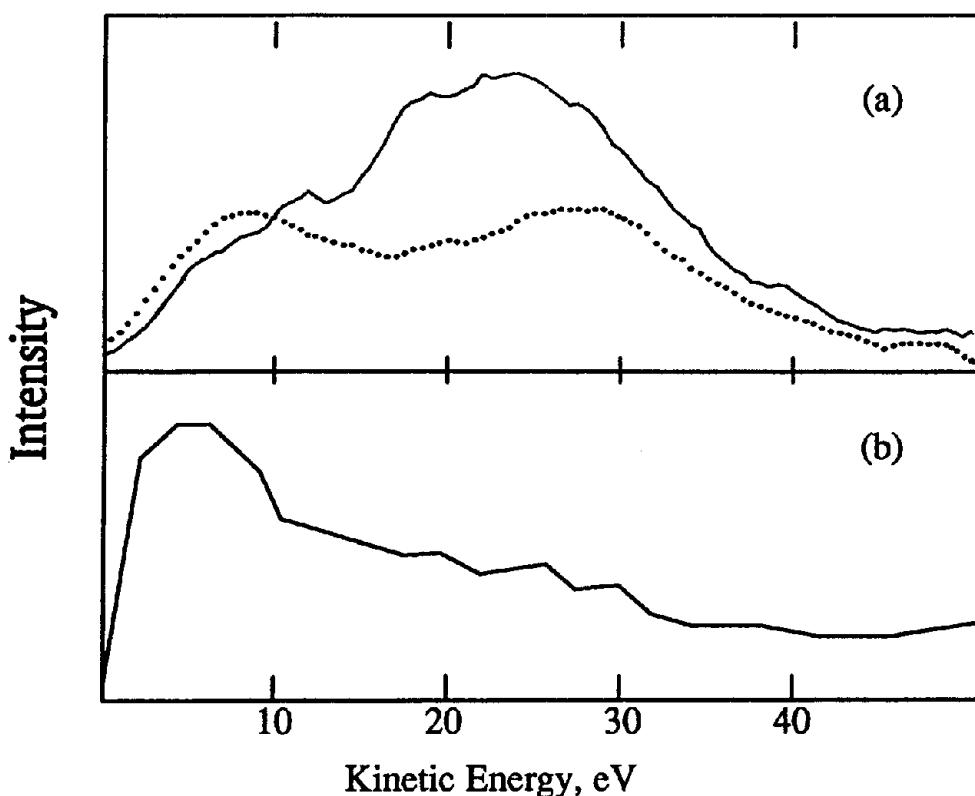
Figure 7. Kinetic energy distributions for \text{Rh}^+ ions (a) and Rh neutral atoms (b) ejected from Rh{111} during bombardment at normal incidence by 3 keV \text{Ar}^+ ions. In (a), the distributions are shown for the \phi = +30^\circ azimuth (solid line) and the -30^\circ azimuth (dotted line). In (b) the +30^\circ azimuth is shown. In all cases, the polar angle of detection is 45^\circ .
