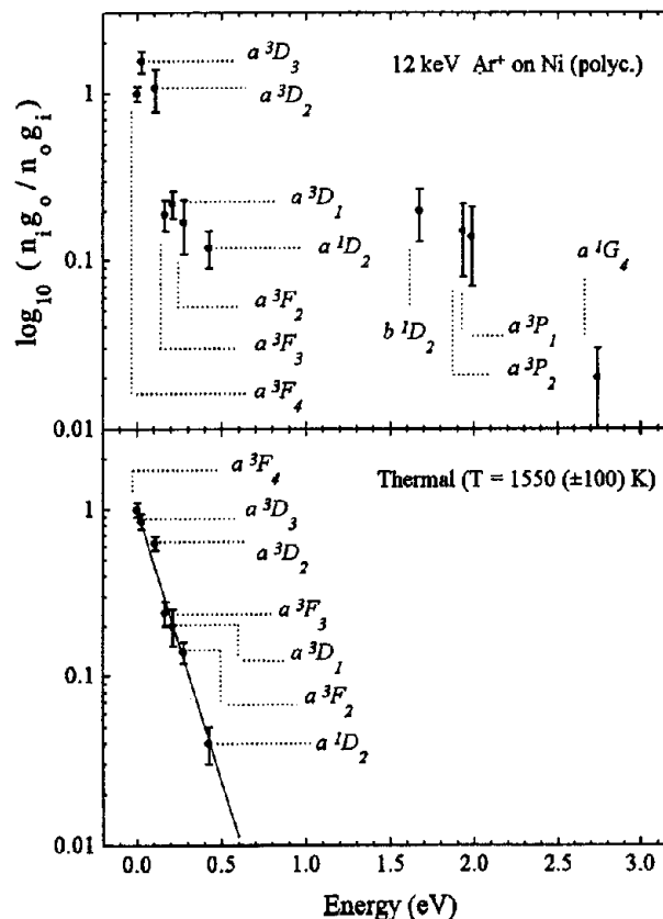
Figure 4. Population distribution of Ni atoms produced by thermal sublimation of a wire (lower frame) and by 12 keV Ar^+ bombardment of a polycrystalline foil (upper frame). The populations ( n_i ) are given relative to the ground state and corrected for the degeneracy of each state ( g_i ). Reprinted from Phys. Rev. Lett. , Vol. 78, E. Vandeweert, V. Philipsen, W. Bouwen, P. Thoen, H. Weidele, R. E. Silverans and P. Lievens, p.138. Copyright 1997, with permission from the American Physical Society.
